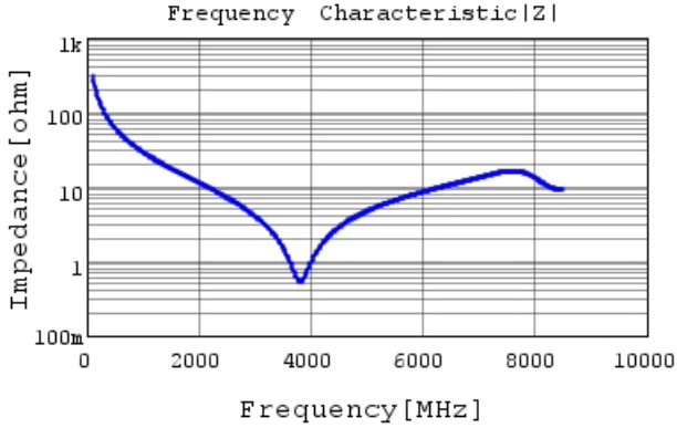
GRM1555C1H5R1BA01 |Z| DC0V, 25degC
