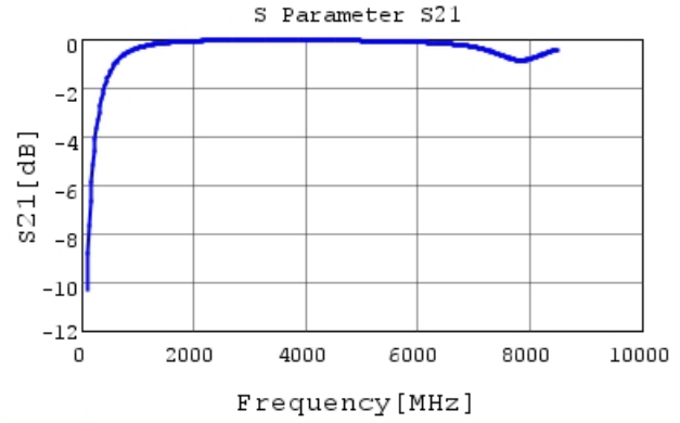
GRM1555C1H5R1BA01 S21 DCOV, 25degC
