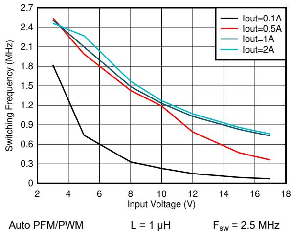
Figure 8-35. Switching Frequency vs Input Voltage V OUT = 1.2 V
