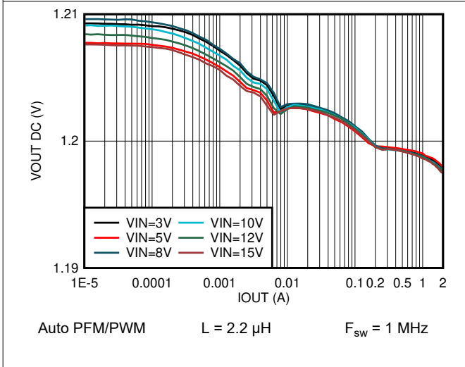
Figure 8-76. Output Voltage vs Output Current V OUT = 1.2 V
