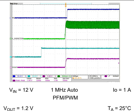
Figure 8-40. Start-up Timing
