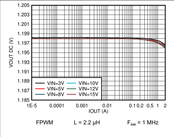
Figure 8-77. Output Voltage vs Output Current V OUT = 1.2 V
