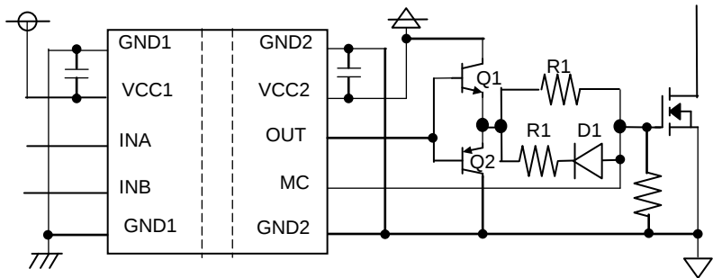
Figure 35. Driving SiC MOSFET with Buffer Circuit
