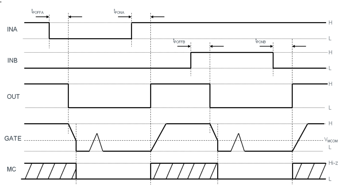
Figure 3. Timing Chart of Miller Clamp Function
