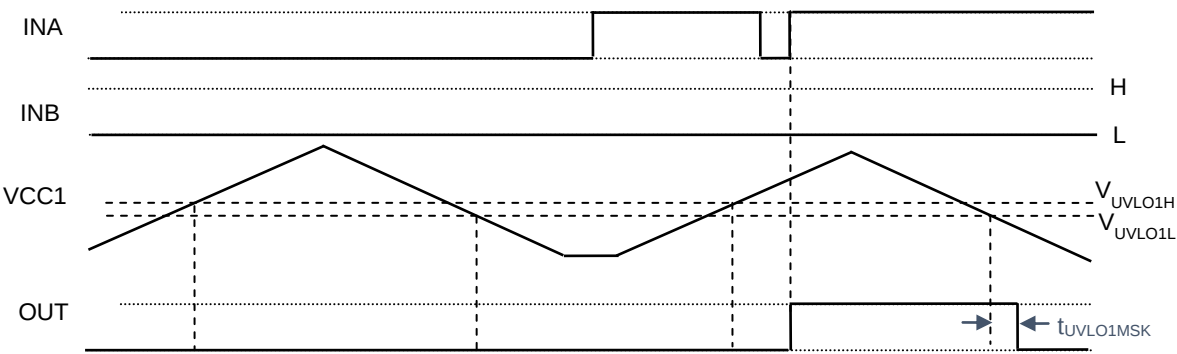
Figure 4. Timing Chart of Input-side UVLO Function
