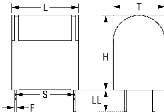
Box with Arc Shape Design (See Ordering Options Note):
