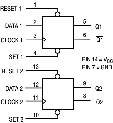
Figure 1. Logic Diagram
