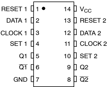
Figure 2. Pinout (Top View)
