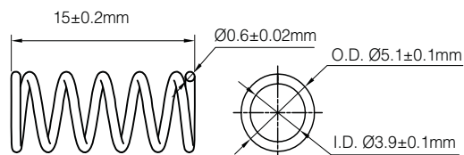
COMPRESSION SPRING:
