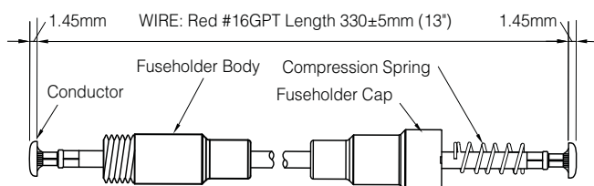
COMPRESSION SPRING:
