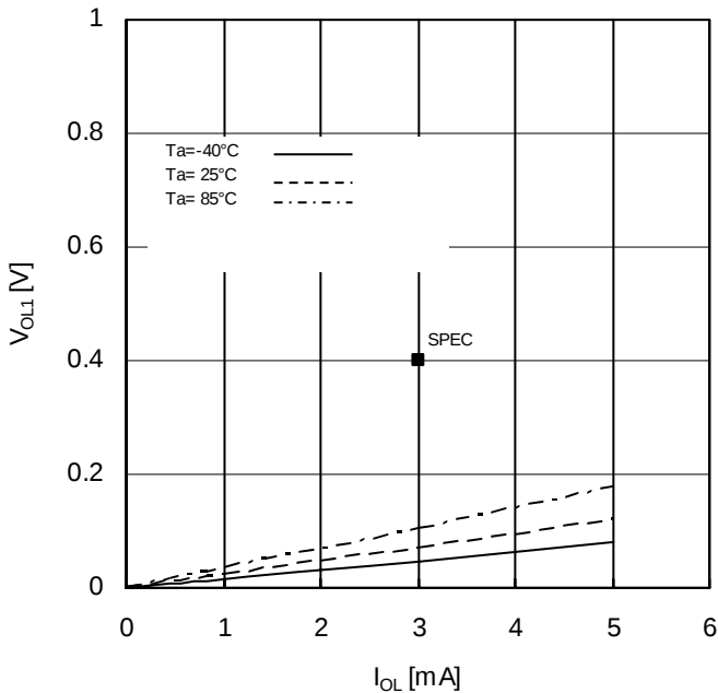
Figure 7. Output Low Voltage1 vs Output Current ( V_{CC}=2.5\text{V} )
