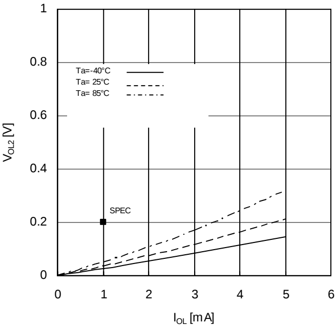
Figure 8. Output Low Voltage2 vs Output Current ( V_{CC}=1.6\text{V} )
