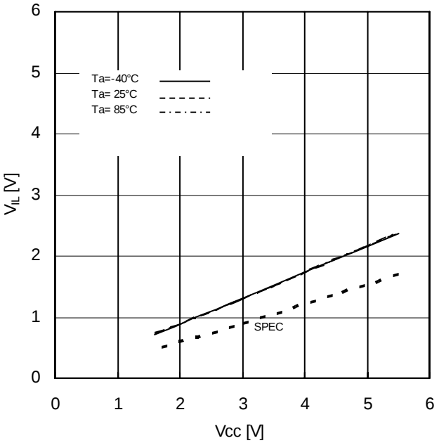
Figure 6. Input Low Voltage1,2 vs Supply Voltage (CSB,SCK,SI,HOLDB,WPB)
