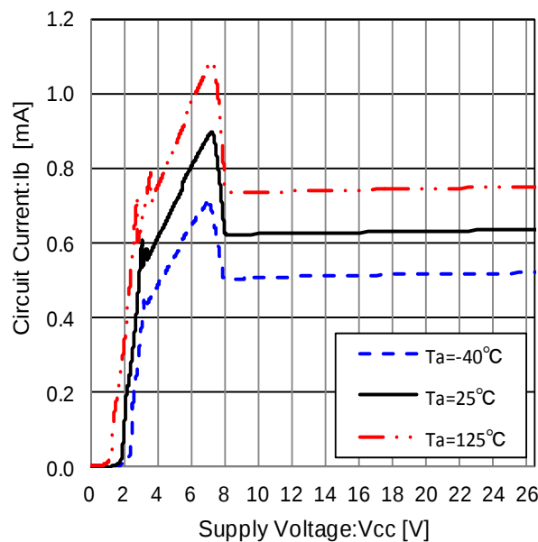
Figure 46. Circuit Current
