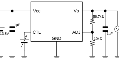
Measurement setup for Figure 21
