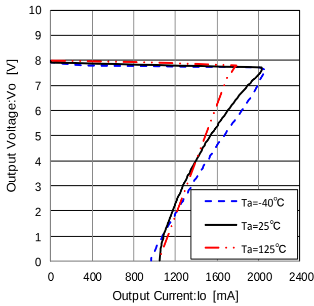
Figure 50. Load Regulation
