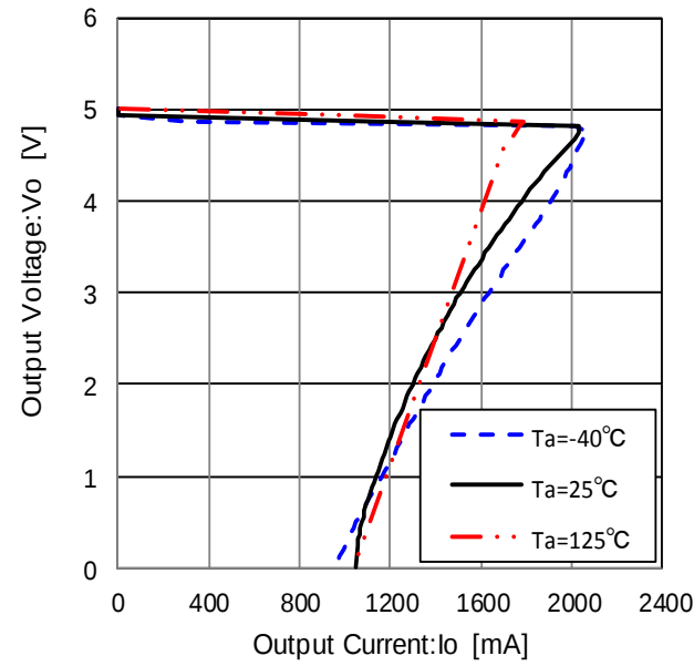
Figure 38. Load Regulation
