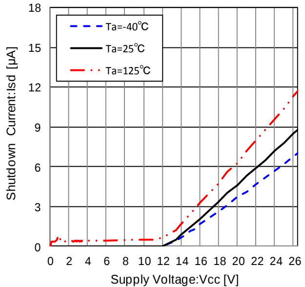
Figure 12. Shutdown Current ( V_{CTL}=0V )
