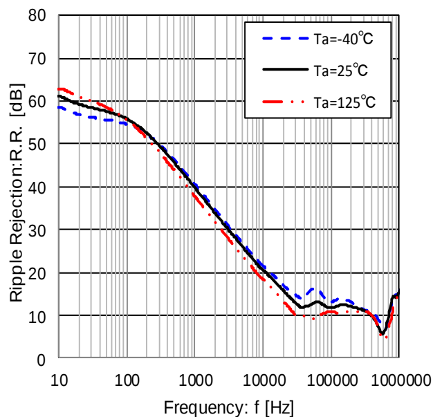
Figure 28. Ripple Rejection ( I_o = 100\text{mA} )
