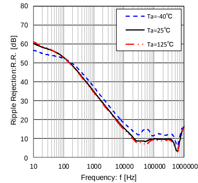
Figure 40. Ripple Rejection ( I_O = 100\text{mA} )
