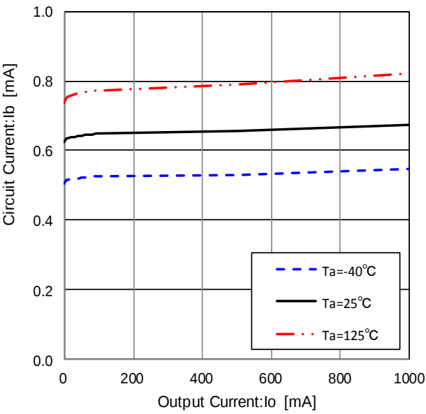
Figure 66. Circuit Current
