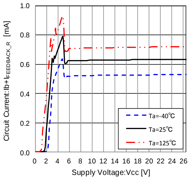
Figure 11. Circuit Current ( I_{FEEDBACK\_R}^{(Note\ 1)} \approx 75\mu A ) (Note 1) I_{FEEDBACK\_R} is the current flowing into external feedback resistance.
