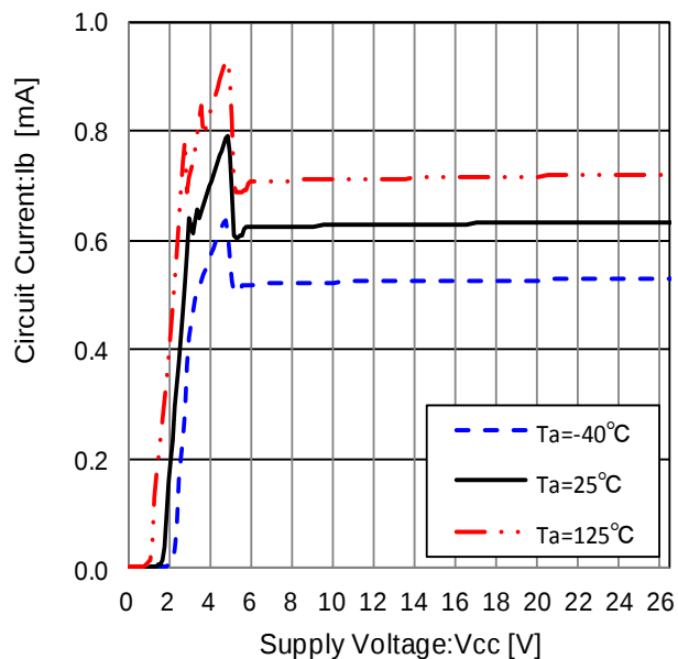
Figure 34. Circuit Current
