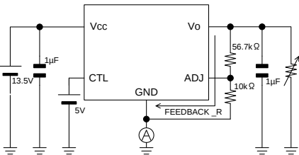
Measurement setup for Figure 19
