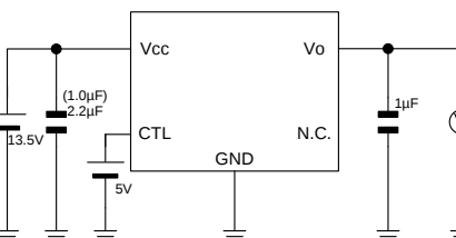
Measurement setup for Figure 29, 41, 53 and 65
