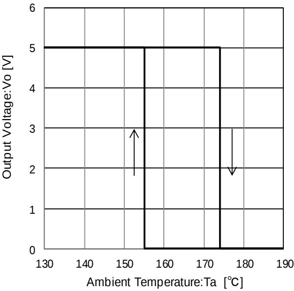
Figure 22. Thermal Shutdown Circuit Characteristic
