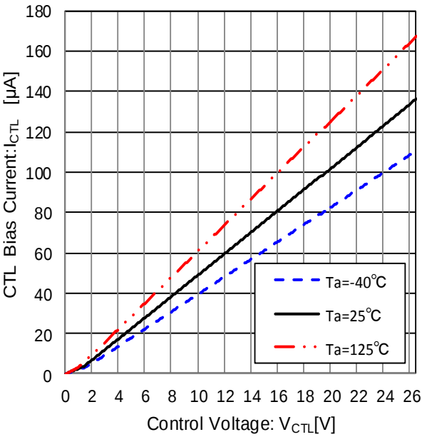
Figure 20. CTL Current vs CTL Voltage
