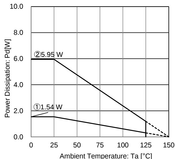
Figure 77. TO263-5 Package Data
