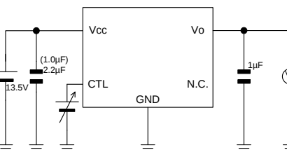
Measurement setup for Figure 32, 44, 56 and 68
