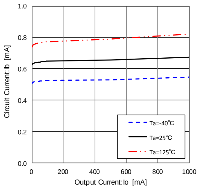
Figure 54. Circuit Current
