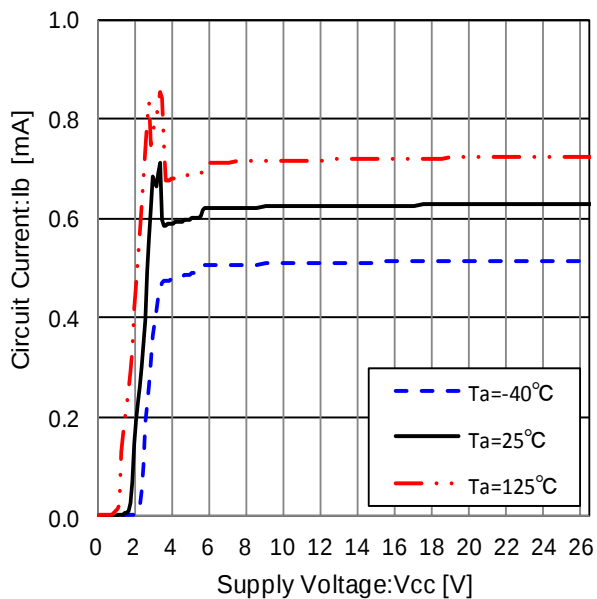
Figure 23. Circuit Current
