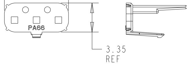
1x3 POSITION
