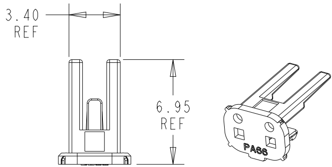
1x2 POSITION
