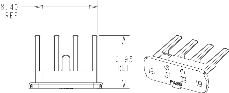
1x4 POSITION
