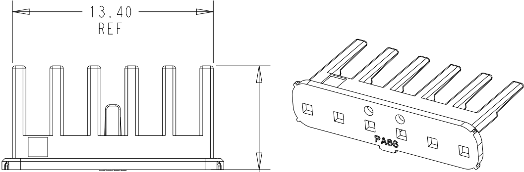
1x6 POSITION
