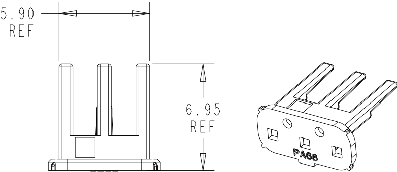
1x3 POSITION
