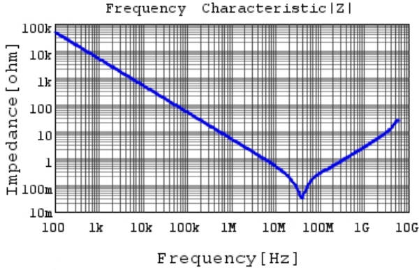
GRM188R71H333KA61 |Z| DCOV, 25degC
