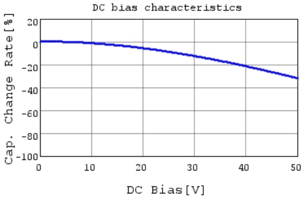
GRM188R71H333KA61 C-DC bias capchange, 25.0c
