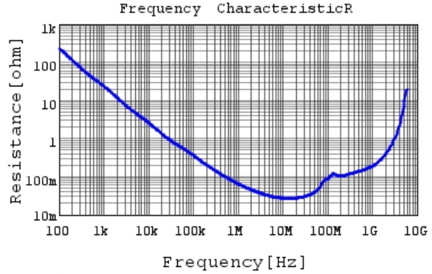
GRM188R71H333KA61 R DCOV, 25degC
