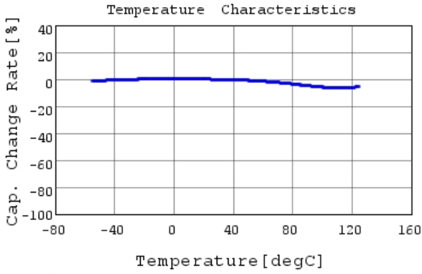
GRM188R71H333KA61 C-Temp. capchange, DC0.0V,
