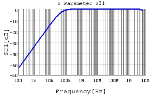
GRM188R71H333KA61 S21 DC0V,25degC
