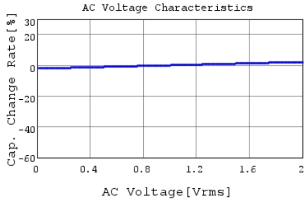
GRM188R71H333KA61 C-AC Voltage capchange, Dc
