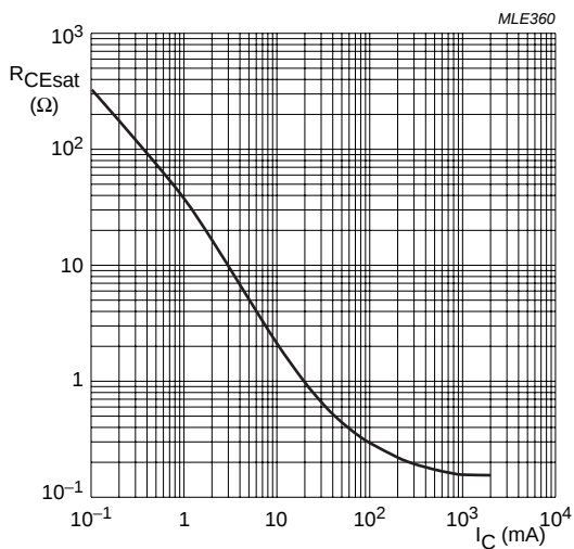
Fig.15 Collector-emitter equivalent on-resistance as a function of collector current; typical values.
