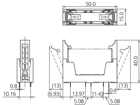
External dimensions
