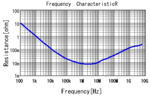
GRM033R60J225ME01 R DCOV, 25degC
