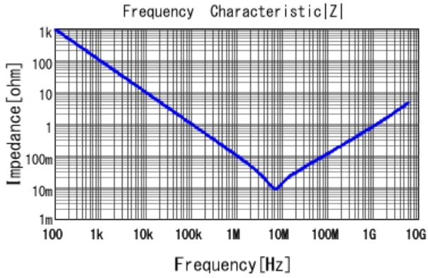
GRM033R60J225ME01 |Z| DCOV, 25degC
