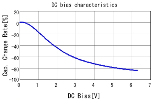
GRM033R60J225ME01 C-DC bias capchange, 25.0degC, A
