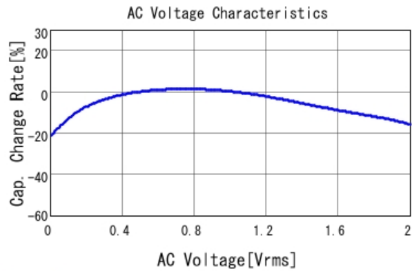
GRM033R60J225ME01 C-AC Voltage capchange, DCOV, 25
