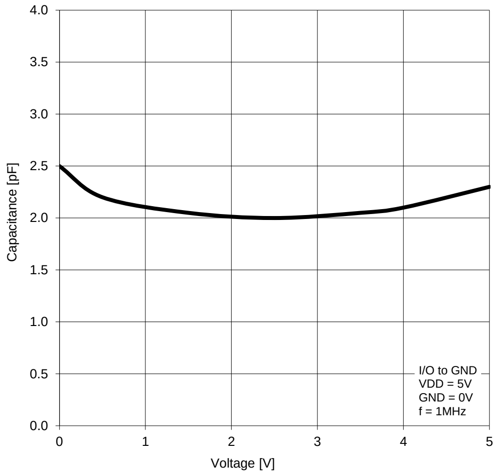
Variation of CIO vs. VI/O:
