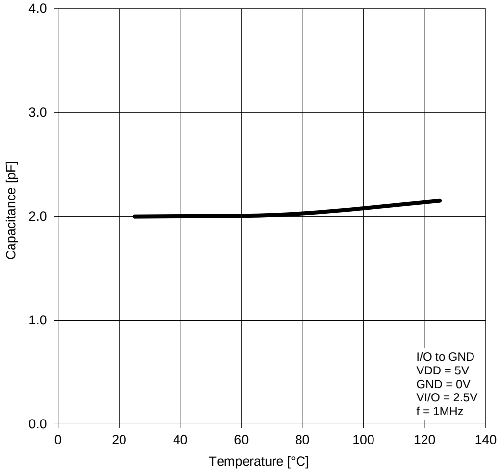
Variation of CIO vs. Temperature:
