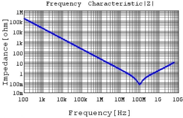
GRM033R61E103MA12 |Z| DCOV, 25degC
