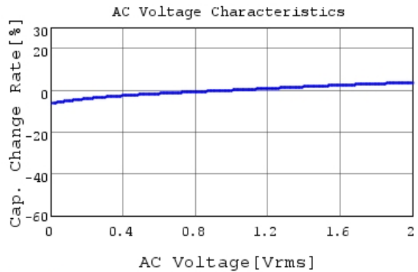
GRM033R61E103MA12 C-AC Voltage capchange, Dc
