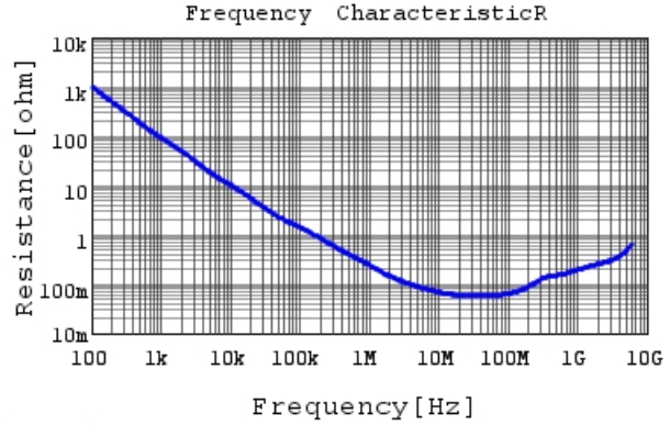
GRM033R61E103MA12 R DCOV, 25degC
