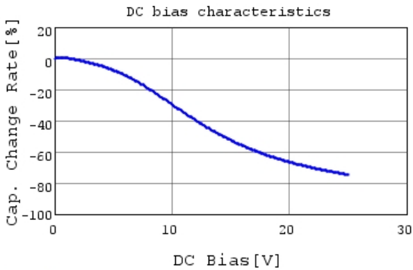
GRM033R61E103MA12 C-DC bias capchange, 25.0c
