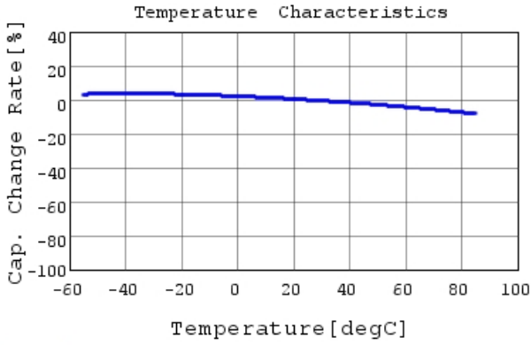
GRM033R61E103MA12 C-Temp. capchange, DC0.0V,
