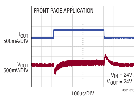
V_{OUT} Transient Response: Load Current Transients from 390mA to 790mA to 390mA
