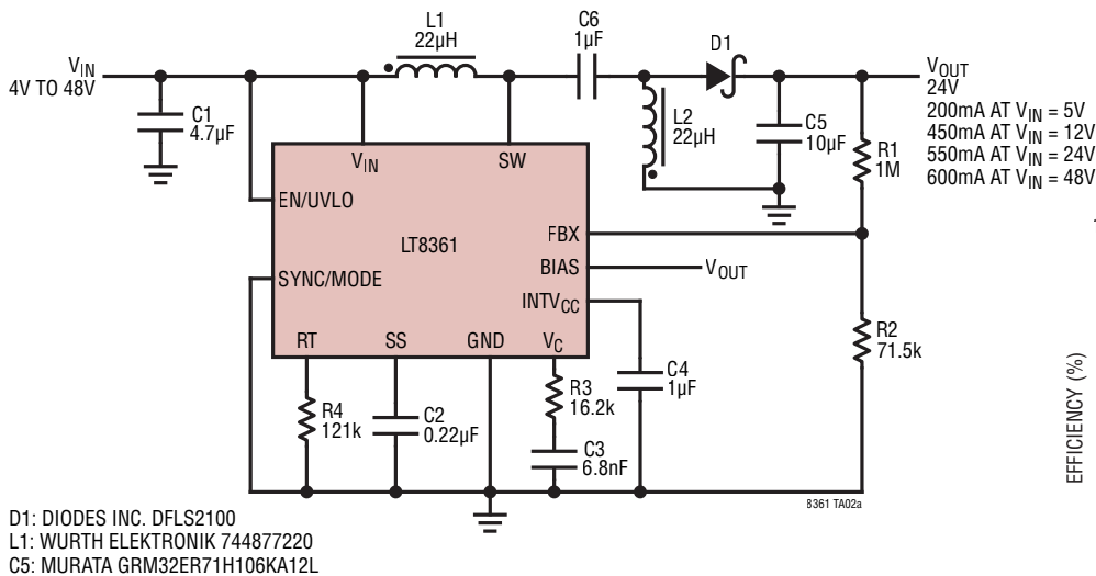
400kHz, 4V to 48V Input, 24V SEPIC Converter
