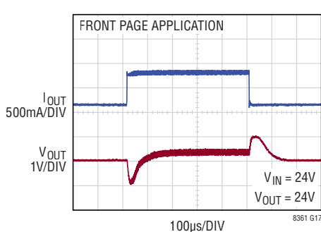
V_{OUT} Transient Response: Load Current Transients from 150mA to 790mA to 150mA
