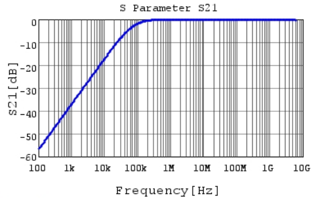
GCM188R71H223KA37 S21 DC0V,25degC
