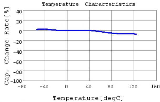
GCM188R71H223KA37 C-Temp. capchange, DC0.0V,
