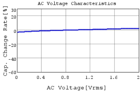
GRM155R71H152KA01 C-AC Voltage capchange, Dc
