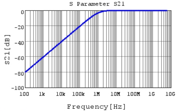
GRM155R71H152KA01 S21 DC0V, 25degC
