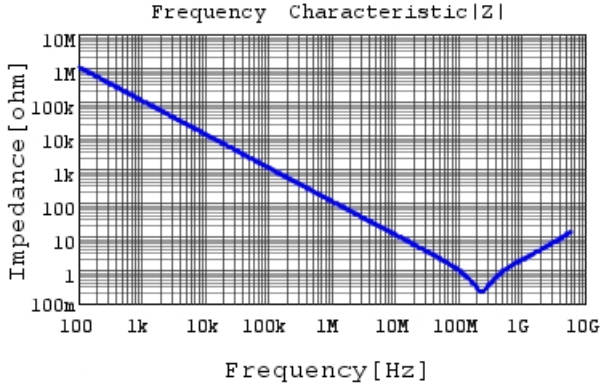
GRM155R71H152KA01 |Z| DCOV,25degC
