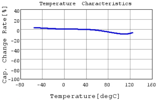
GRM155R71H152KA01 C-Temp. capchange, DC0.0V,
