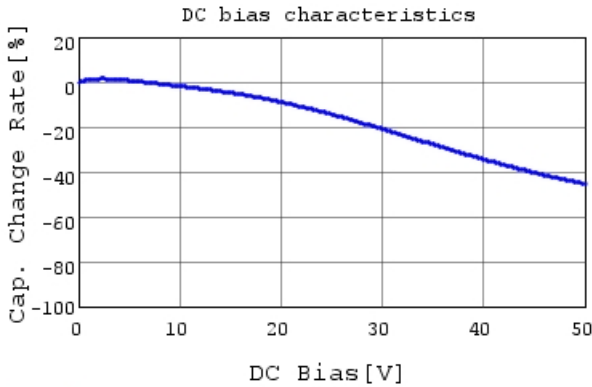
GRM155R71H152KA01 C-DC bias capchange, 25.0c
