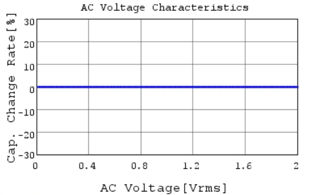
GRT1555C2A101JA02 C-AC Voltage capchange, Dc
