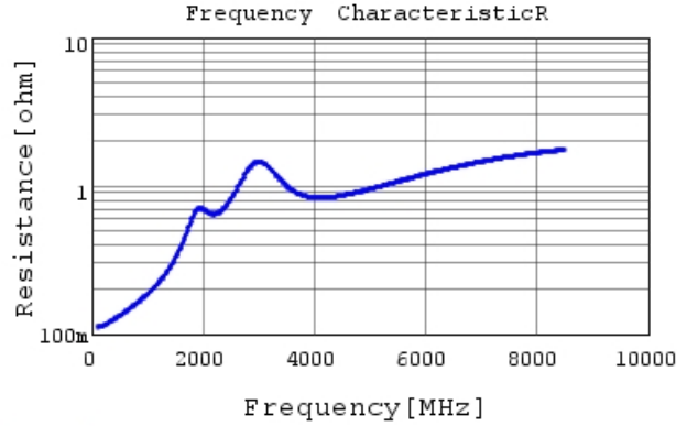
GRT1555C2A101JA02 R DCOV, 25degC
