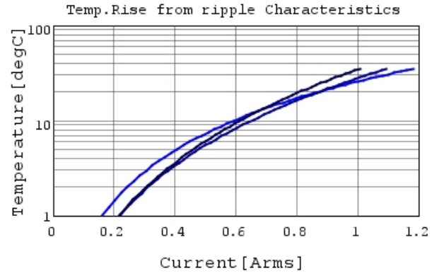
GRM1555C1H820GA01 Temp.rise 200MHz
