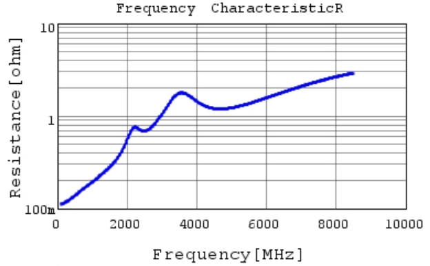
GRM1555C1H820GA01 R DC0V, 25degC
