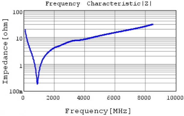
GRM1555C1H820GA01 |Z| DC0V, 25degC
