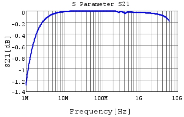
GCM1885C1H272JA16 S21 DCOV, 25degC
