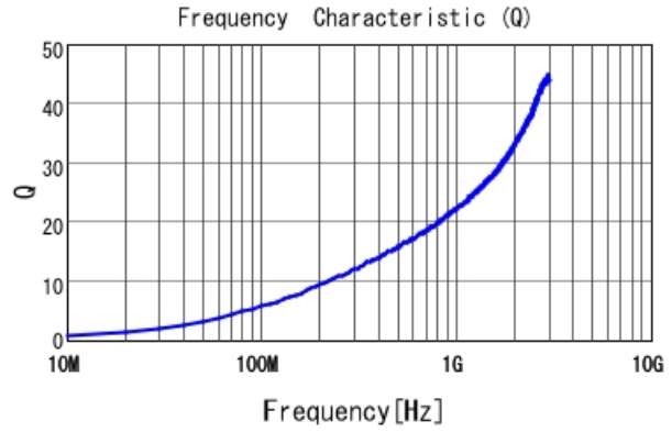
LQP02TQ2N4B02 Q
