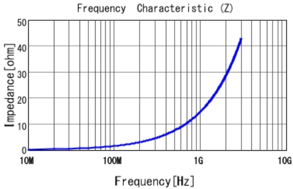
LQP02TQ2N4B02 |Z|
