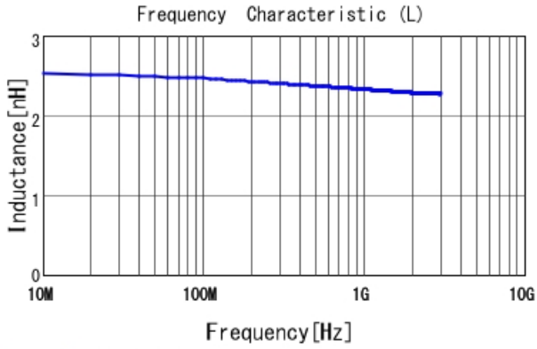
LQP02TQ2N4B02 L
