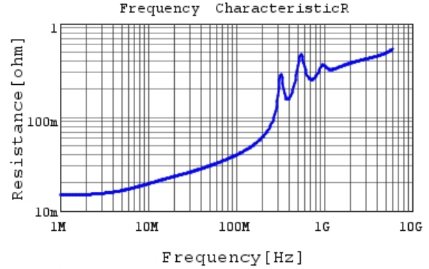
GRM1885C1H202JA01 R DCOV, 25degC
