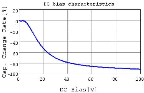
GRM155R62A104ME14 C-DC bias capchange, 25.0c
