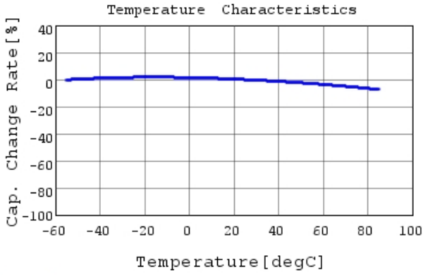
GRM155R62A104ME14 C-Temp. capchange, DC0.0V,
