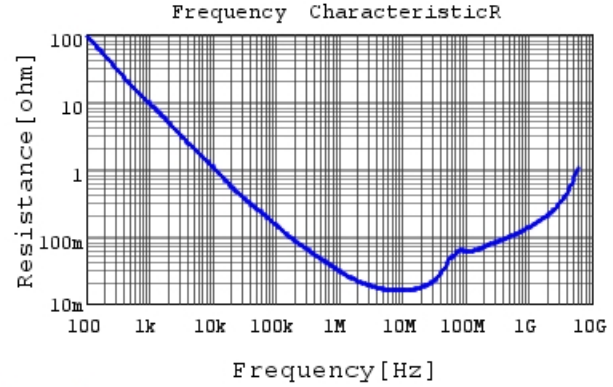
GRM155R62A104ME14 R DCOV, 25degC
