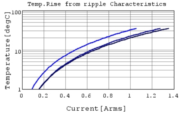
GRM155R62A104ME14 Temp.rise — 400kHz —
