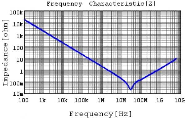
GRM155R62A104ME14 |Z| DCOV, 25degC
