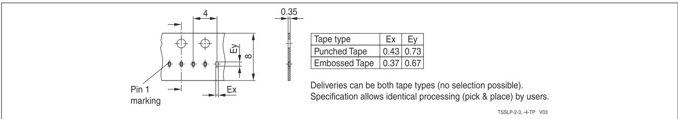
Figure 12 TSSLP-2-4 packing
