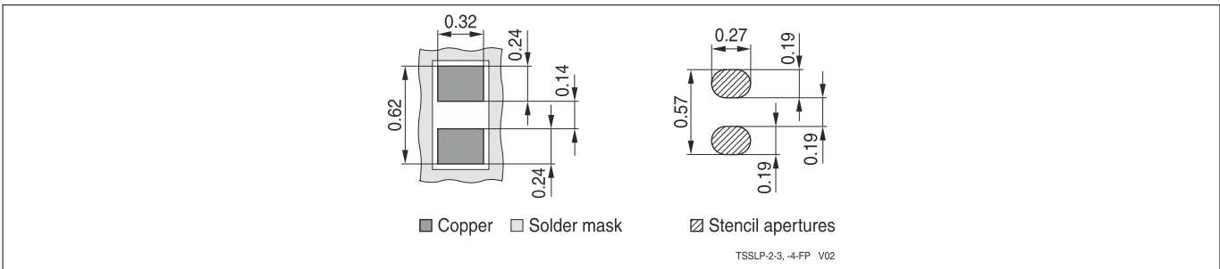
Figure 11 TSSLP-2-4 footprint
