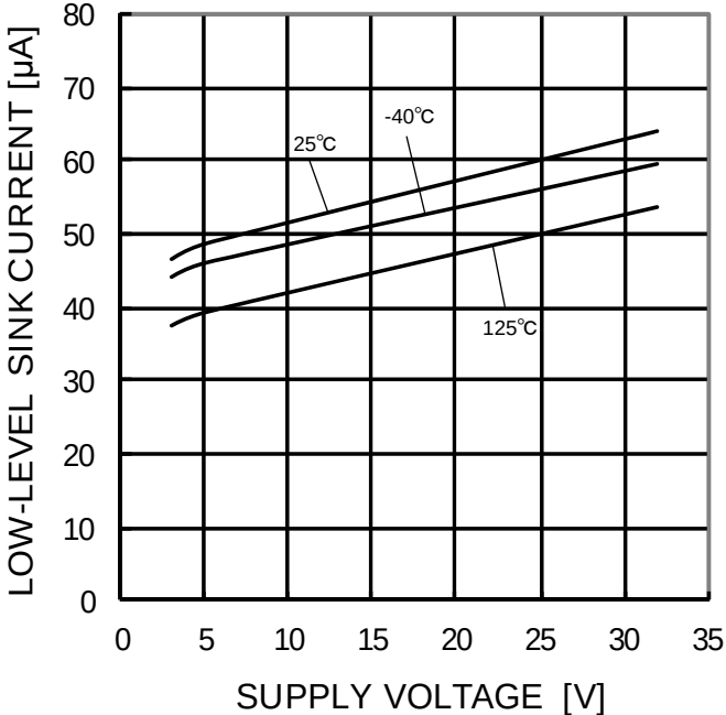
Figure 35. Low Level Sink Current – Supply Voltage (OUT=0.2V)
