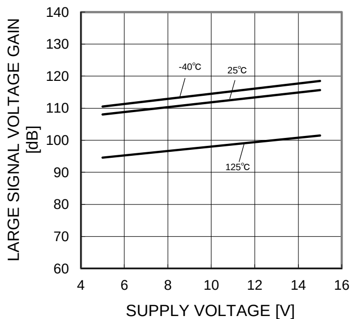
Figure 21. Large Signal Voltage Gain – Supply Voltage (R L =2kΩ)
