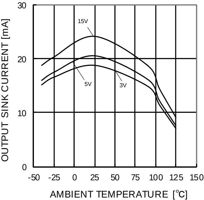
Figure 34. Output Sink Current – Ambient Temperature (OUT=VCC)
