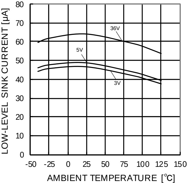
Figure 36. Low Level Sink Current – Ambient Temperature (OUT=0.2V)
