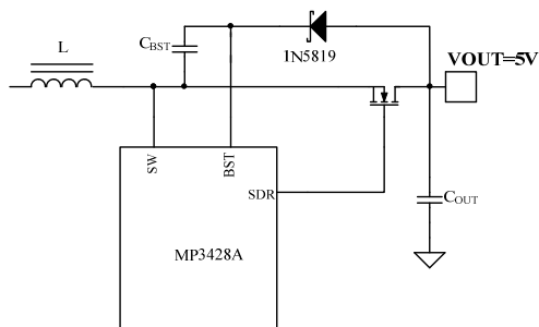
Figure 3: BST Charger for Low Output Application
