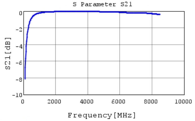
GRM1555C1H6R8CA01 S21 DCOV, 25degC
