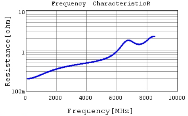
GRM1555C1H6R8CA01 R DCOV, 25degC
