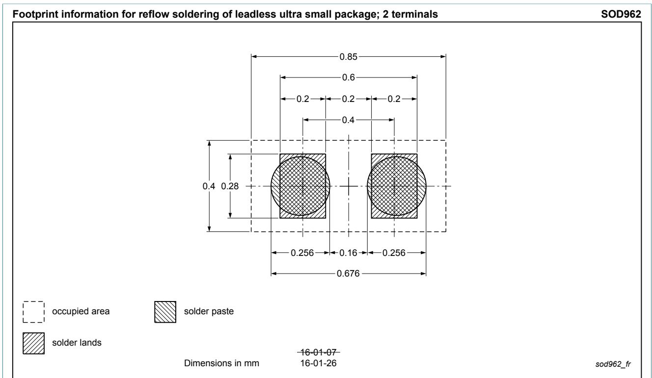
Fig. 22. Reflow soldering footprint for DSN0603-2 (SOD962)
