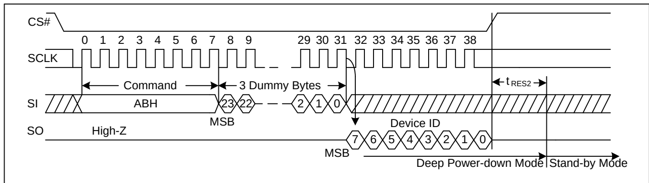
Figure 60. Release Power-Down/Read Device ID Sequence Diagram
