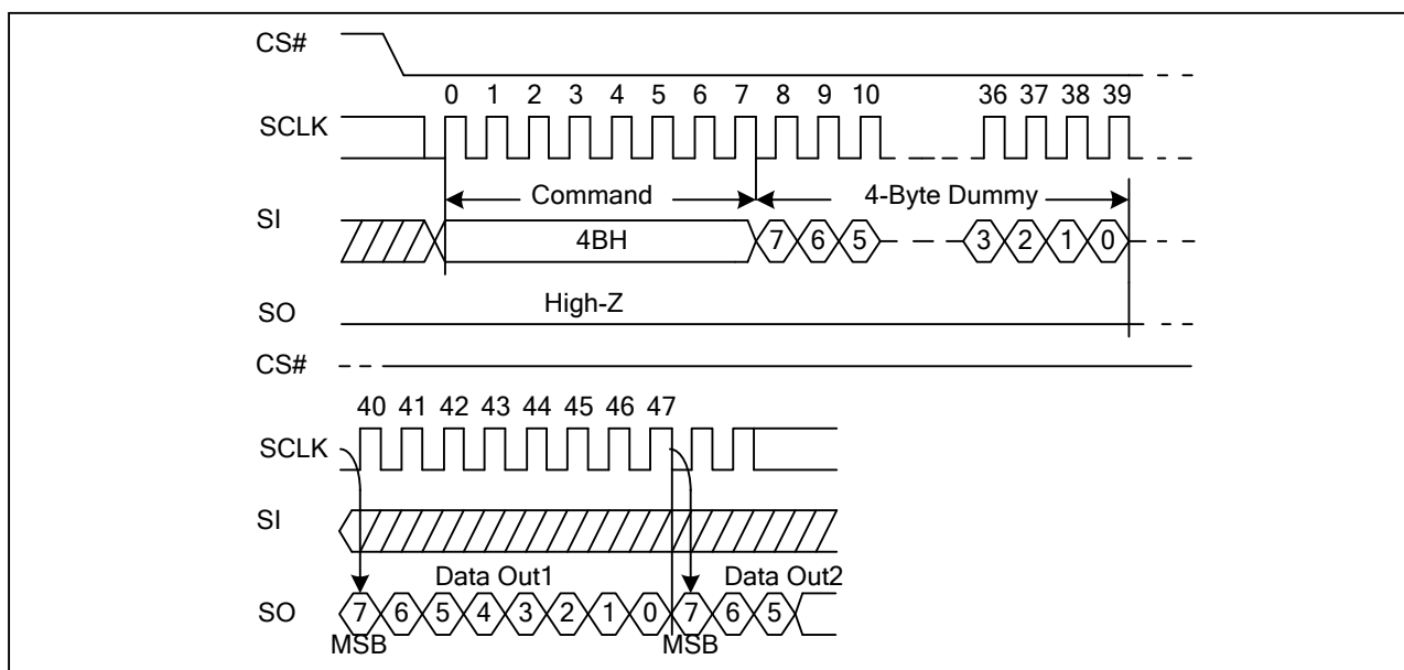
Figure 55. Read Unique ID Sequence Diagram (ADS=1)
