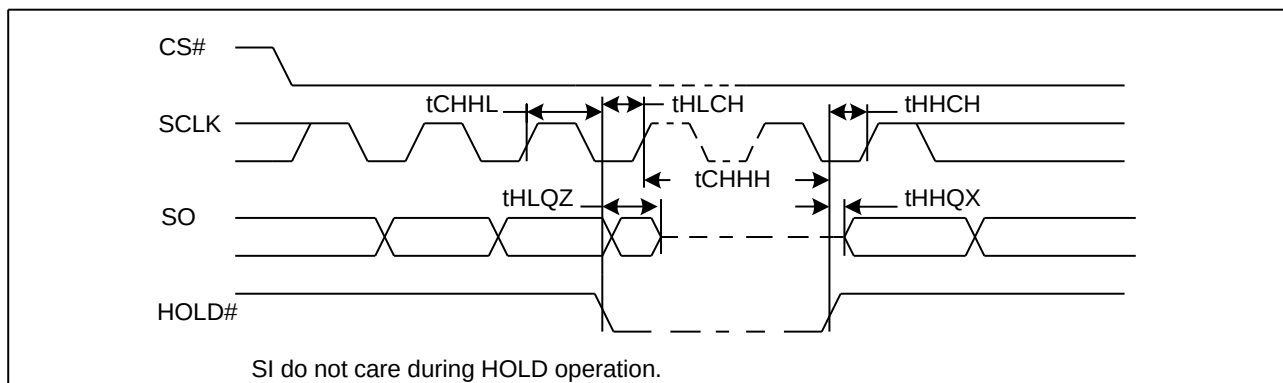
Figure 81 Hold Timing
