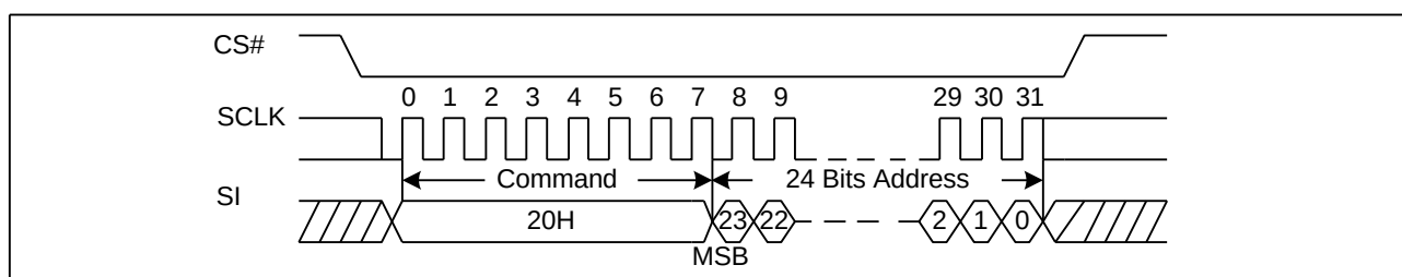
Figure 43. Sector Erase Sequence Diagram (ADS=0)
