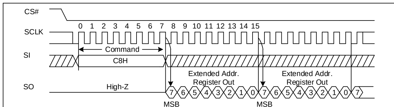
Figure 10 Read Extended Register Sequence Diagram
