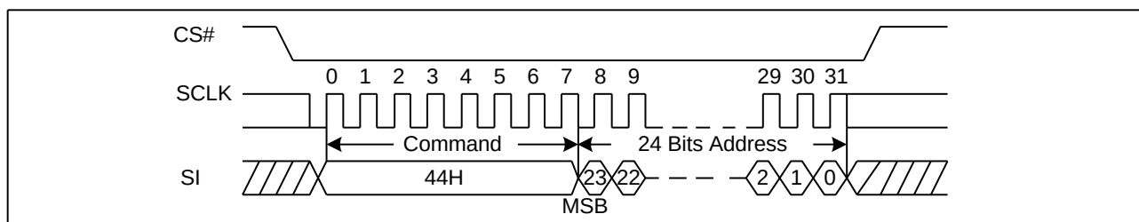
Figure 67. Erase Security Registers command Sequence Diagram (ADS=0)
