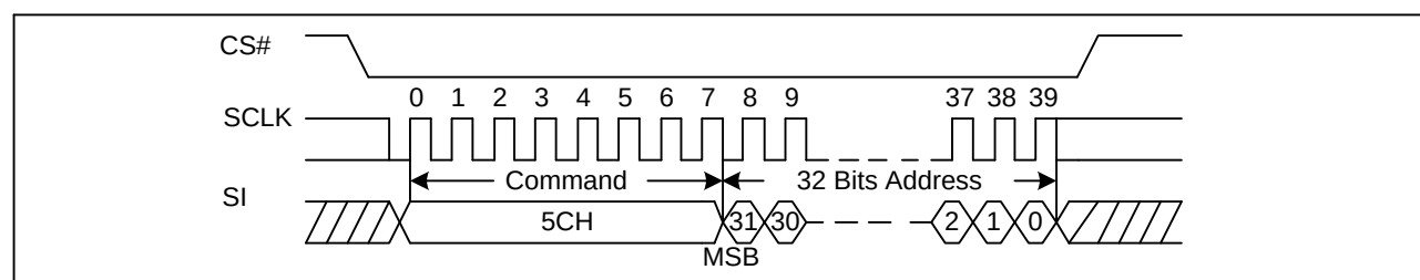
Figure 48. 32KB Block Erase with 4-Byte Address Sequence Diagram (ADS=0 or ADS=1)
