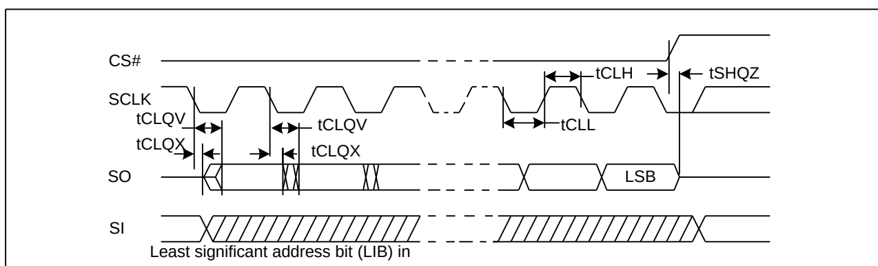
Figure 79. Output Timing
