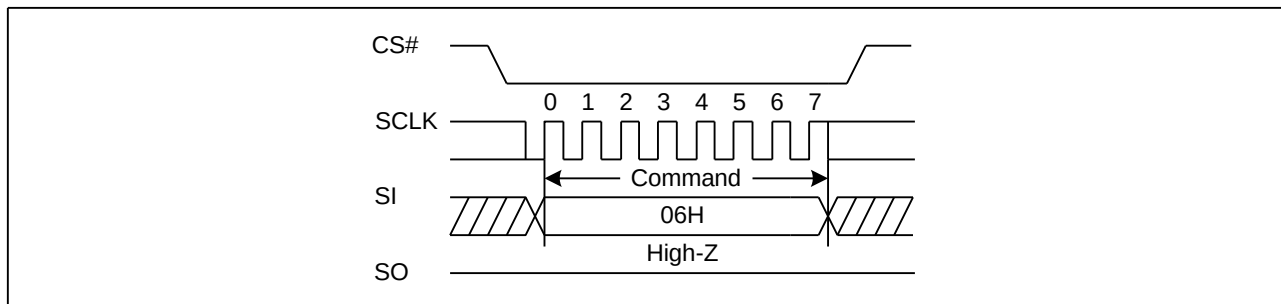
Figure 5. Write Enable Sequence Diagram
