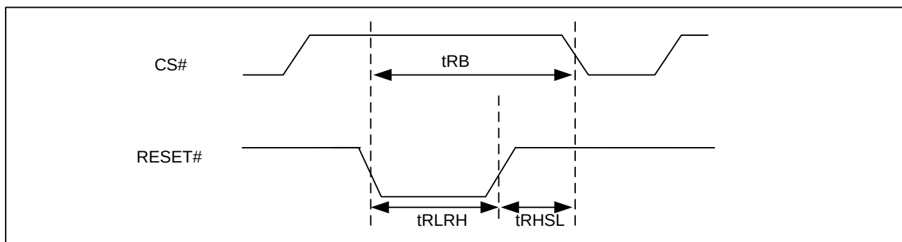
Figure82. RESET Timing
