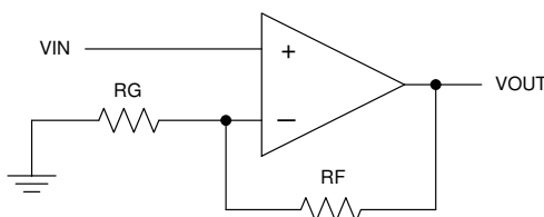
Figure 10-1. Schematic Representation
