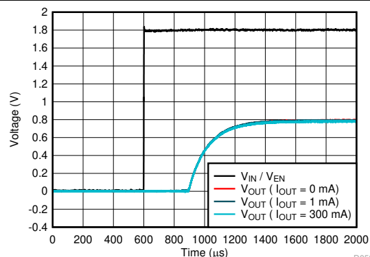
Figure 6-74. Start-Up
