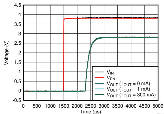
Figure 6-76. Start-Up
