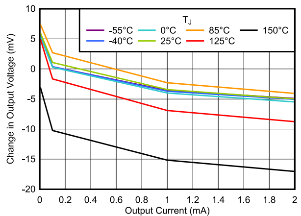
Figure 6-10. Load Regulation vs I_{OUT}
