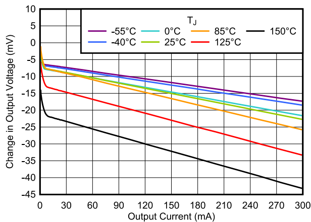
Figure 6-9. Load Regulation vs I_{OUT}
