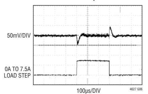
1.0V Transient Response
