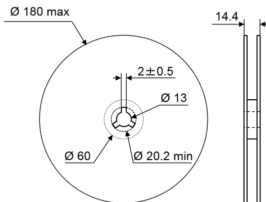
Figure 14. Reel dimensions (mm)
