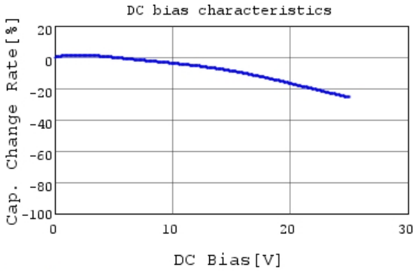
GRM155R71E682KA01 C-DC bias capchange, 25.0c
