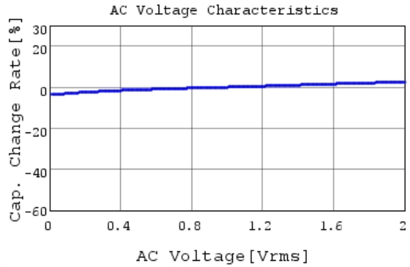
GRM155R71E682KA01 C-AC Voltage capchange, Dc
