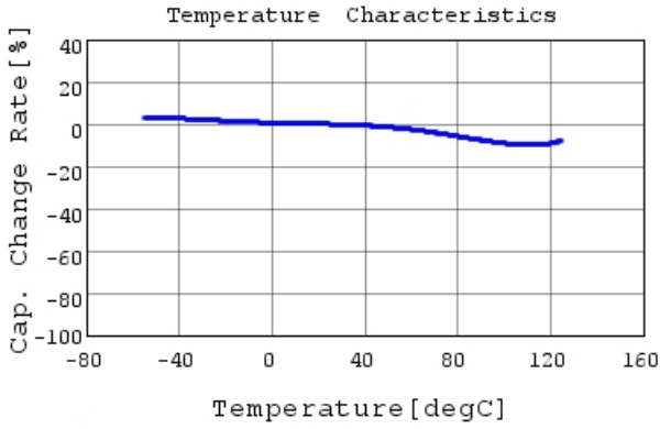
GRM155R71E682KA01 C-Temp. capchange, DC0.0V,
