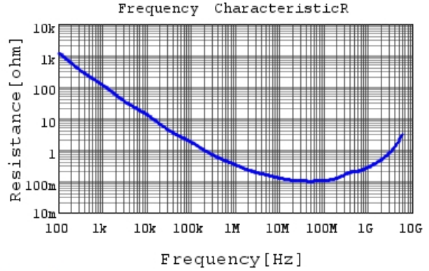
GRM155R71E682KA01 R DCOV, 25degC
