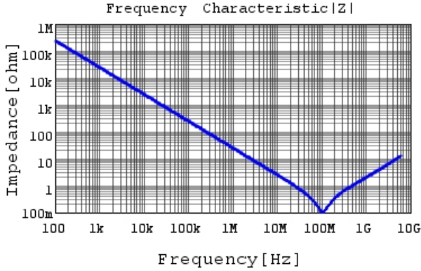
GRM155R71E682KA01 |Z| DCOV, 25degC
