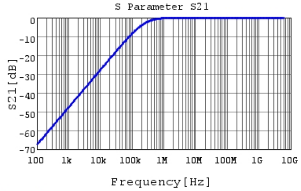
GRM155R71E682KA01 S21 DC0V, 25degC
