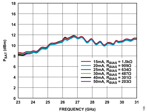
Figure 35. P_{SAT} vs. Frequency for Various I_{DQ} and R_{BIAS} Values, V_{DD} = 2\text{ V}
