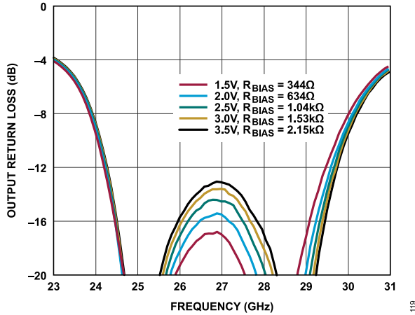
Figure 19. Output Return Loss vs. Frequency for Various Supply Voltages and R_{BIAS} Values, I_{DQ} = 25\text{ mA}
