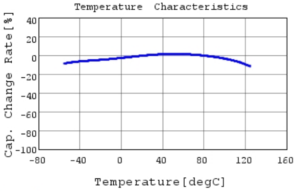
GCJ21BR71E225KA01 C-Temp. capchange, DC0.0V,
