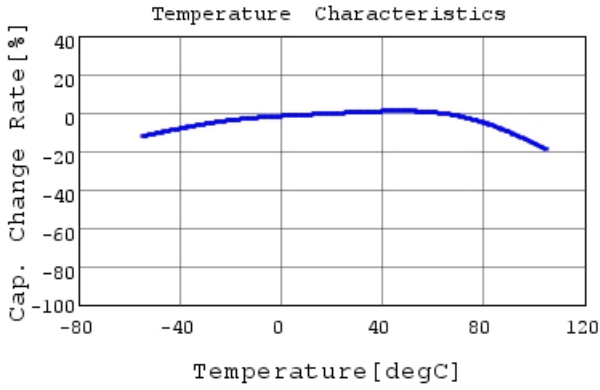
GRM155C80J106ME18 C-Temp. capchange, DC0.0V,
