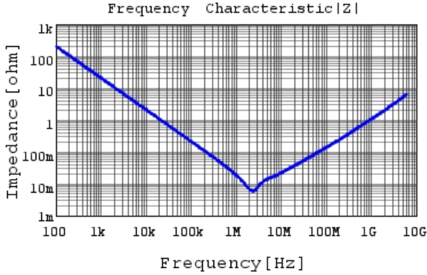
GRM155C80J106ME18 |Z| DCOV, 25degC
