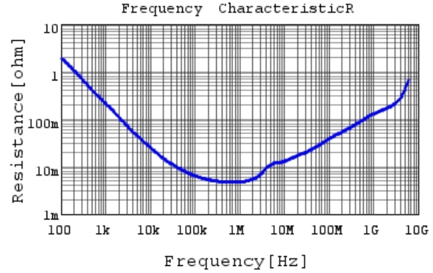
GRM155C80J106ME18 R DCOV, 25degC
