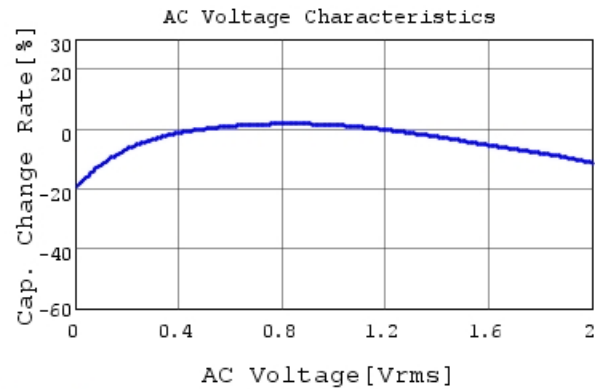
GRM155C80J106ME18 C-AC Voltage capchange, Dc
