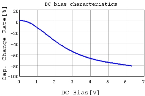
GRM155C80J106ME18 C-DC bias capchange, 25.0c
