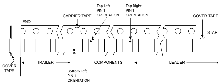
Figure 8-4 Tape leader and Trailer Pin 1 Orientation
