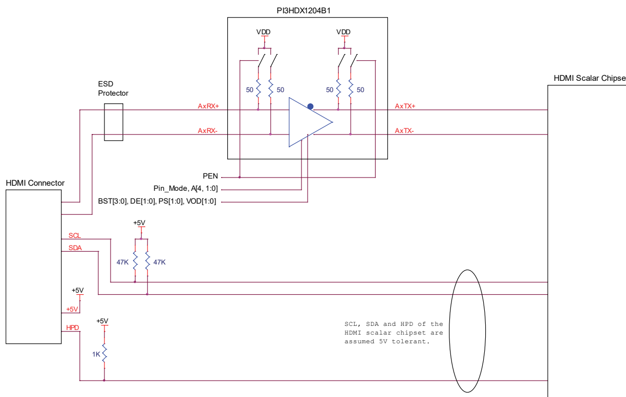
Figure 7-6 PI3HDX1204B1 Sink Application Circuit
