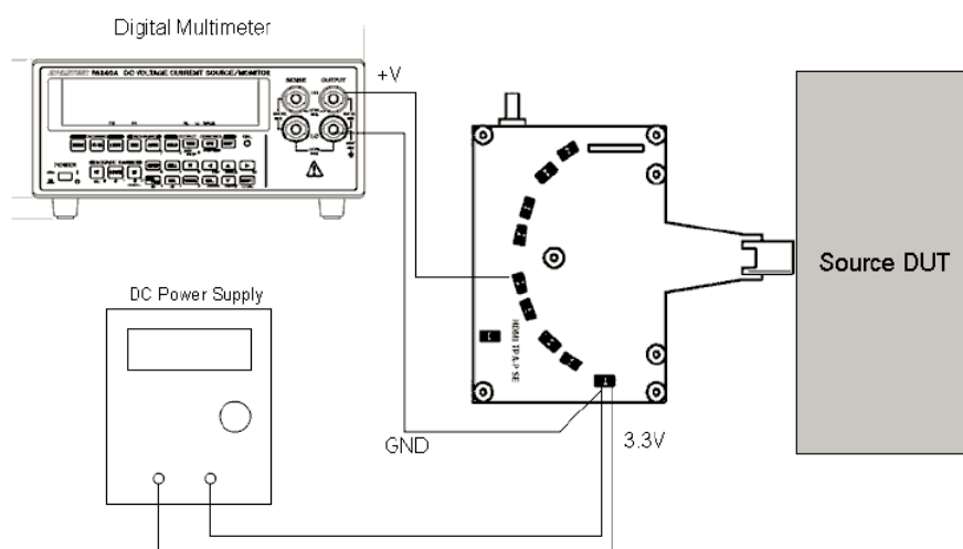
Figure 7-3 HDMI VOFF Test Setup
