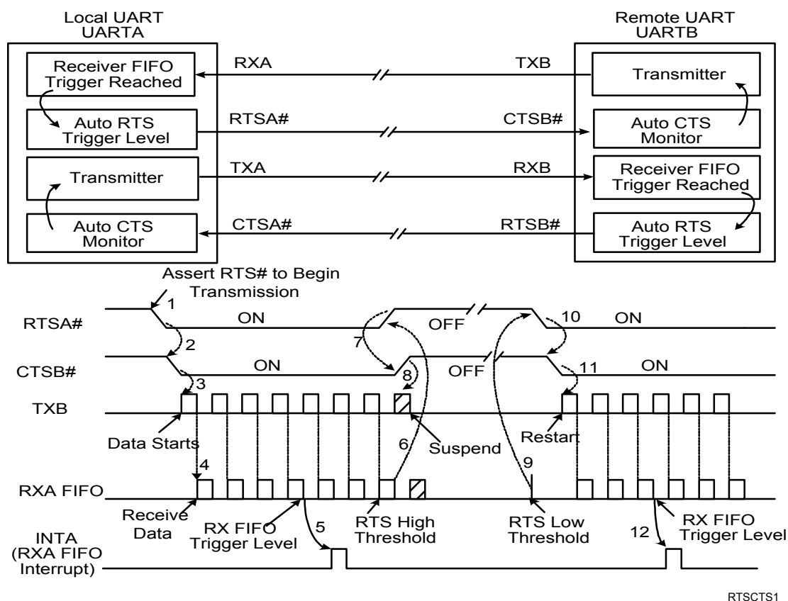
FIGURE 11. AUTO RTS/DTR AND CTS/DSR FLOW CONTROL OPERATION
