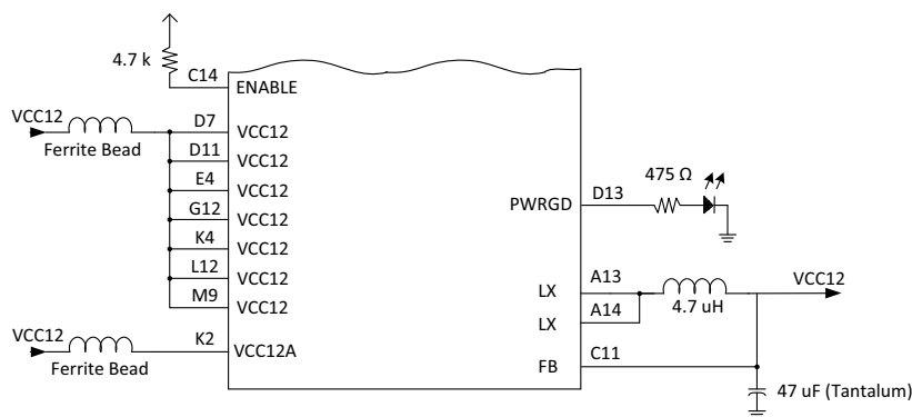
FIGURE 3. BUCK REGULATOR
