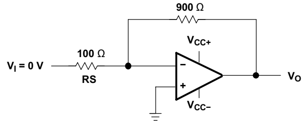
Figure 8-2. Noise-Test Circuit
