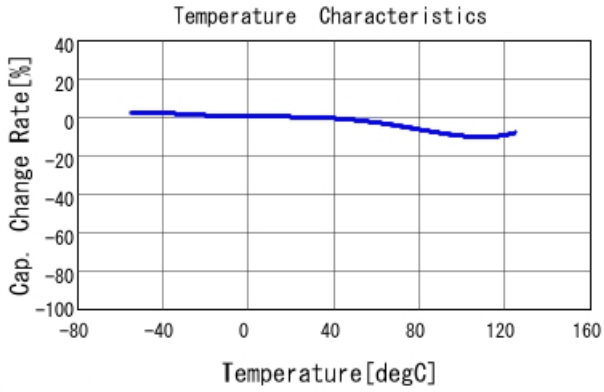
GRM155R11H222KA01 C-Temp. capchange, DC0.0V, AC1.C
