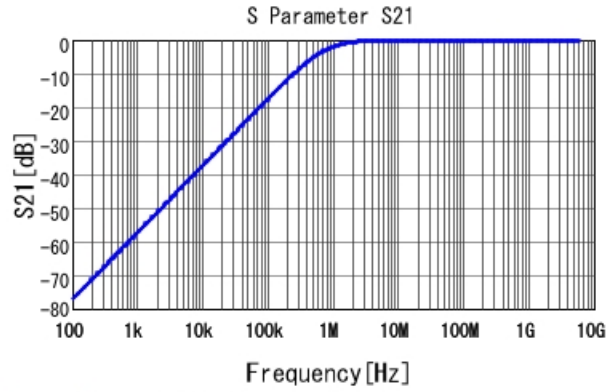
GRM155R11H222KA01 S21 DC0V, 20degC
