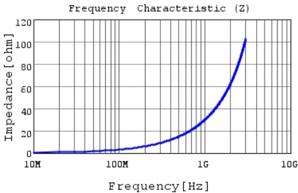
LQP15MN4N7B02 |Z|
