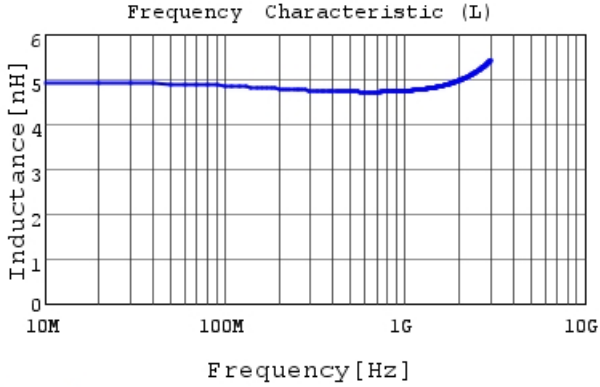
LQP15MN4N7B02 L
