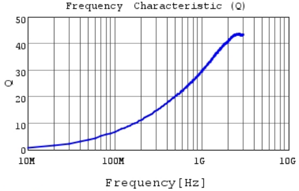
LQP15MN4N7B02 Q
