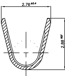
SECTION "B-B" SCALE 10/1
