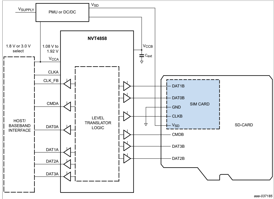
Figure 8. Application circuit interfacing with typical SD or SIM card
