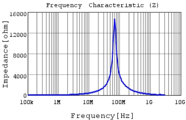
LQH2MPZ6R8MGR |Z|
