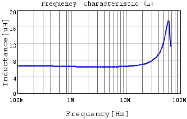
LQH2MPZ6R8MGR L
