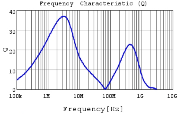
LQH2MPZ6R8MGR Q
