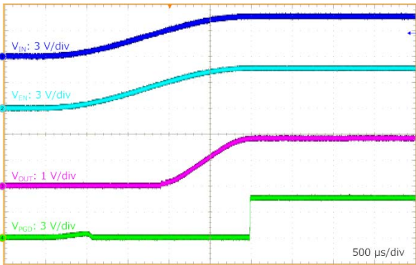
Figure 60. VIN Start-up at No Load (VIN = VEN = 0 V to 5 V, VOUT = 1.8 V)
