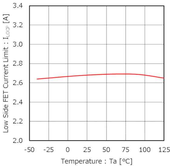
Figure 13. Low Side FET Current Limit vs Temperature
