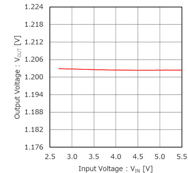
Figure 42. Output Voltage vs Input Voltage (Line Regulation) (VOUT = 1.2 V, IOUT = 1.0 A)
