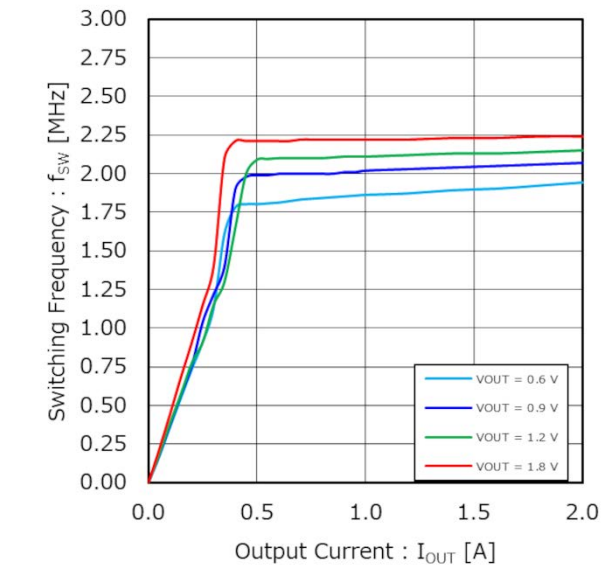
Figure 40. Switching Frequency vs Output Current (VIN = 3.3 V)
