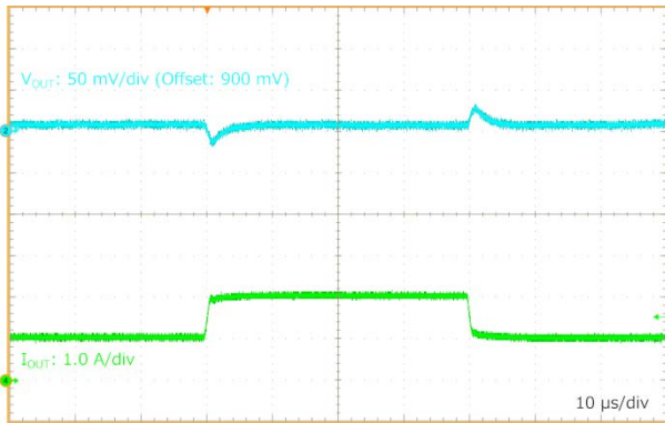
Figure 53. Load Transient Response ( V_{IN} = 3.3\text{ V} , V_{OUT} = 0.9\text{ V} , I_{OUT} = 1.0\text{ A} to 2.0\text{ A} : 1\text{ A}/\mu\text{s} )
