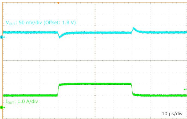
Figure 55. Load Transient Response ( V_{IN} = 5.0\text{ V} , V_{OUT} = 1.8\text{ V} , I_{OUT} = 1.0\text{ A} to 2.0\text{ A} : 1\text{ A}/\mu\text{s} )
