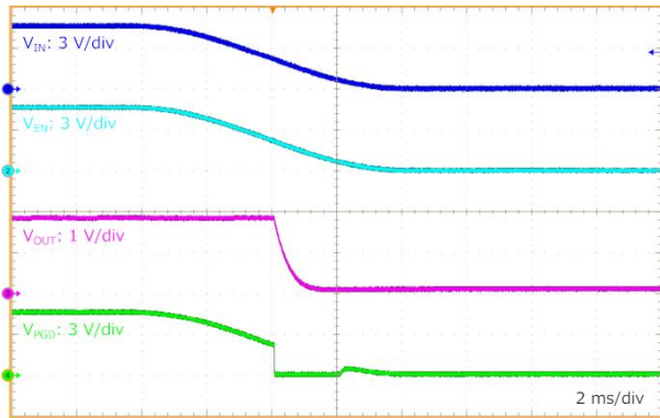
Figure 61. VIN Shutdown at No Load (VIN = VEN = 5 V to 0 V, VOUT = 1.8 V)
