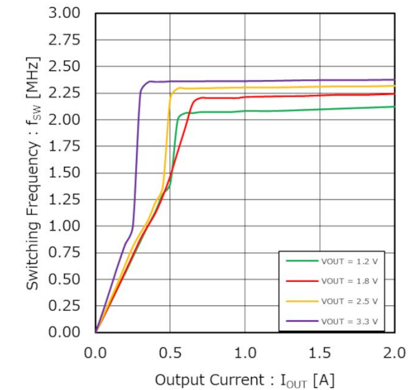
Figure 41. Switching Frequency vs Output Current (VIN = 5.0 V)
