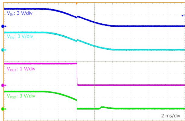
Figure 63. VIN Shutdown at RLoad = 0.9 Ω (VIN = VEN = 5 V to 0 V, VOUT = 1.8 V)
