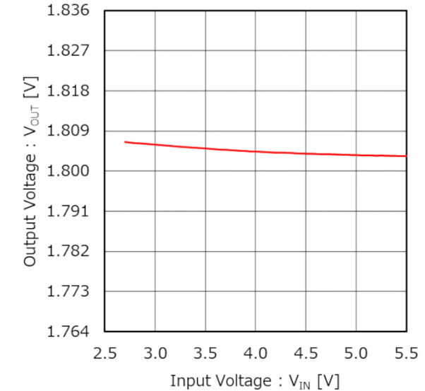
Figure 43. Output Voltage vs Input Voltage (Line Regulation) (VOUT = 1.8 V, IOUT = 1.0 A)
