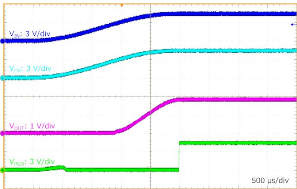
Figure 62. VIN Start-up at RLoad = 0.9 Ω (VIN = VEN = 0 V to 5 V, VOUT = 1.8 V)
