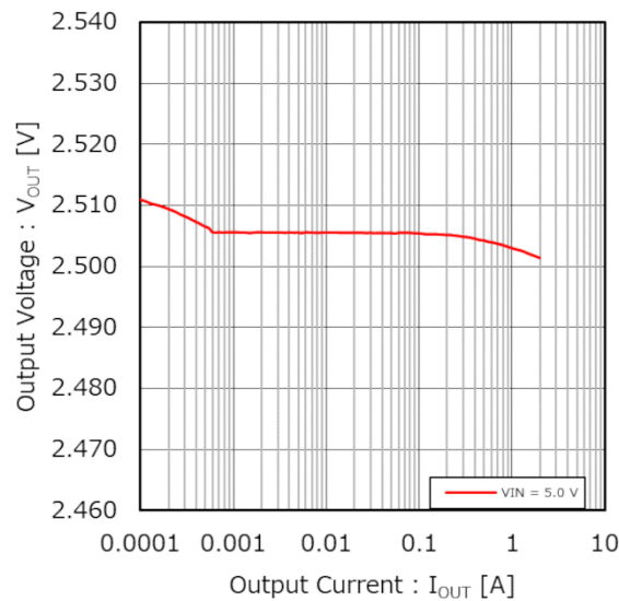
Figure 38. Output Voltage vs Output Current (Load Regulation) ( V_{OUT} = 2.5 V)
