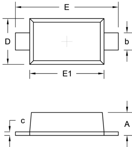
SOD-123F
