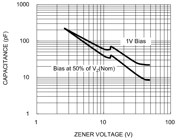
Fig.5 Typical Capacitance
