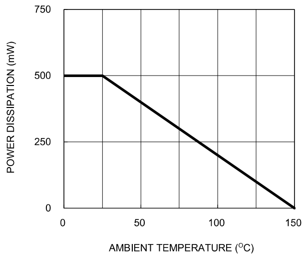
Fig.4 Power Dissipation Curve
