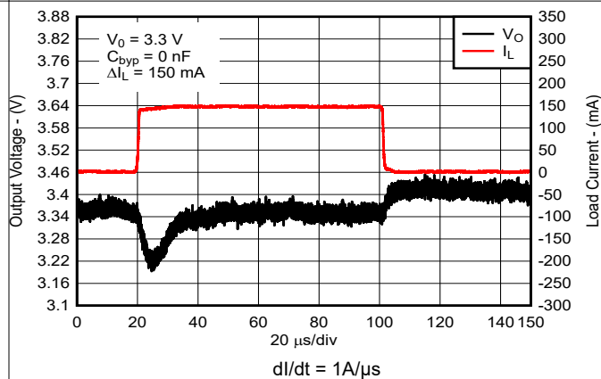
Figure 5-40. Load Transient Response (New Chip)
