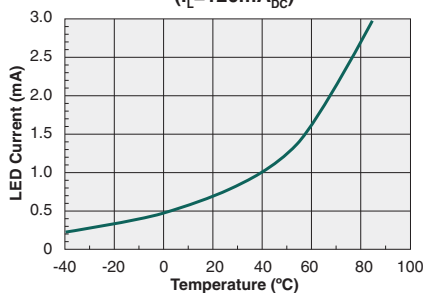
Typical I_F for Switch Dropout vs. Temperature ( I_L = 120\text{mA}_{\text{DC}} )
