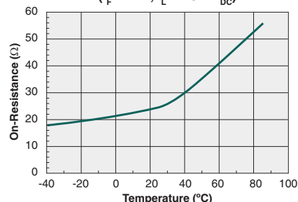
Typical On-Resistance vs. Temperature ( I_F = 2\text{mA} , I_L = 120\text{mA}_{\text{DC}} )
