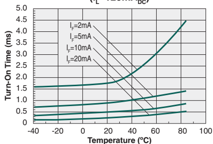
Typical Turn-On Time vs. Temperature ( I_L = 120\text{mA}_{\text{DC}} )
