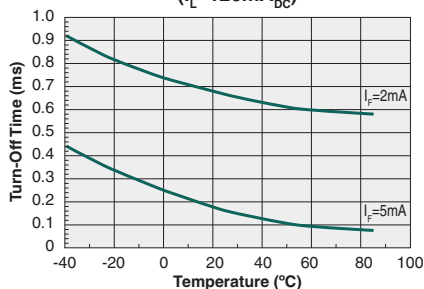
Typical Turn-Off Time vs. Temperature ( I_L = 120\text{mA}_{\text{DC}} )
