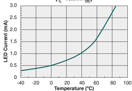
Typical I_F for Switch Operation vs. Temperature ( I_L = 120\text{mA}_{\text{DC}} )
