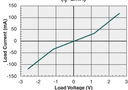
Typical Load Current vs. Load Voltage ( I_F = 2\text{mA} )
