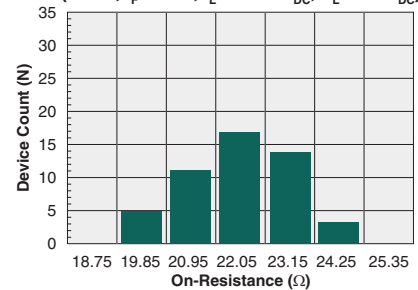
Typical On-Resistance Distribution (N=50, I_F=2\text{mA} , I_L=120\text{mA}_{DC} , V_L=350\text{V}_{DC} )
